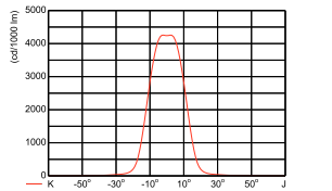
OFCC_BBP623 GC 34xLED-HB/NW MB-Cartesian Outdoor (combined)
