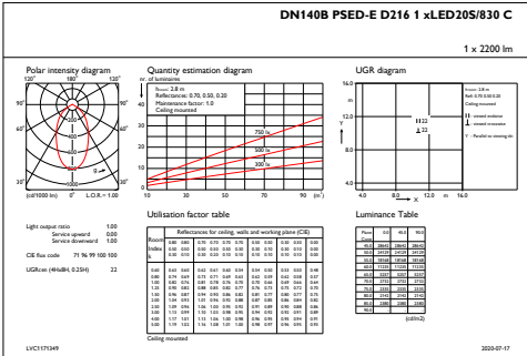
IFGU1_DN140BPSED-ED2161xLED20S830C
