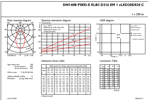
IFGU1_DN140BPSED-EELB3D216EM1xLED20S830C
