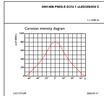
IFCC1_DN140BPSED-ED2161xLED20S830C
