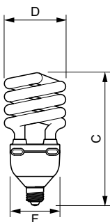
Tornado High Lumen 45W WW E27 1CT/6
