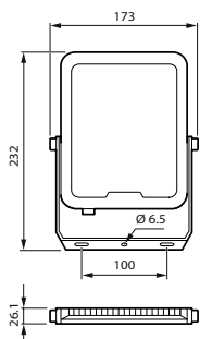
BVP164 LED60/865 PSU 50W SWB CE
