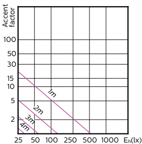
MASTER LEDspotMV 35W GU10 922-927 36D
